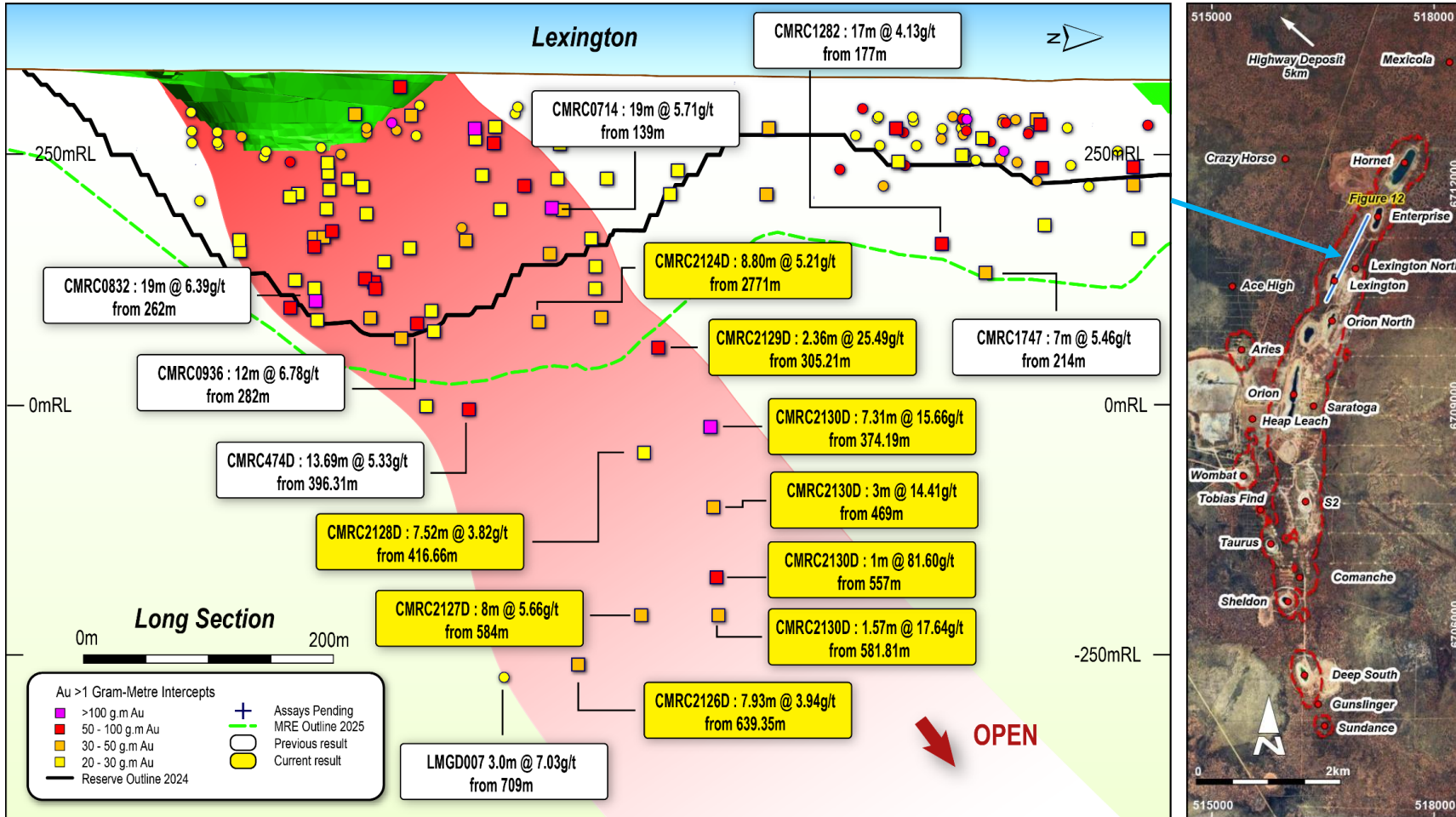
Long section with +550m of prospective north plunging strike of recently identified +20 gram metre intercepts and pending assays located along the Orion mine tend at Lexington looking west, with significant high-grade mineralisation outside of the current A$2,200/oz reserve outline and A$2,400/oz resource outline.
