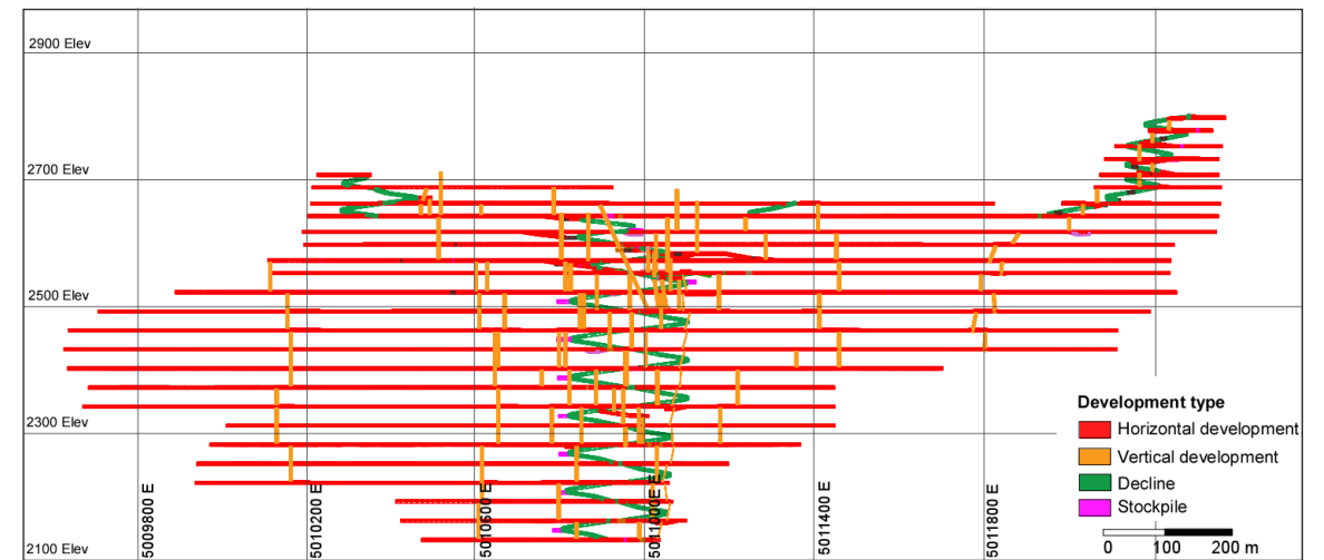
Long Section of Mine Design
