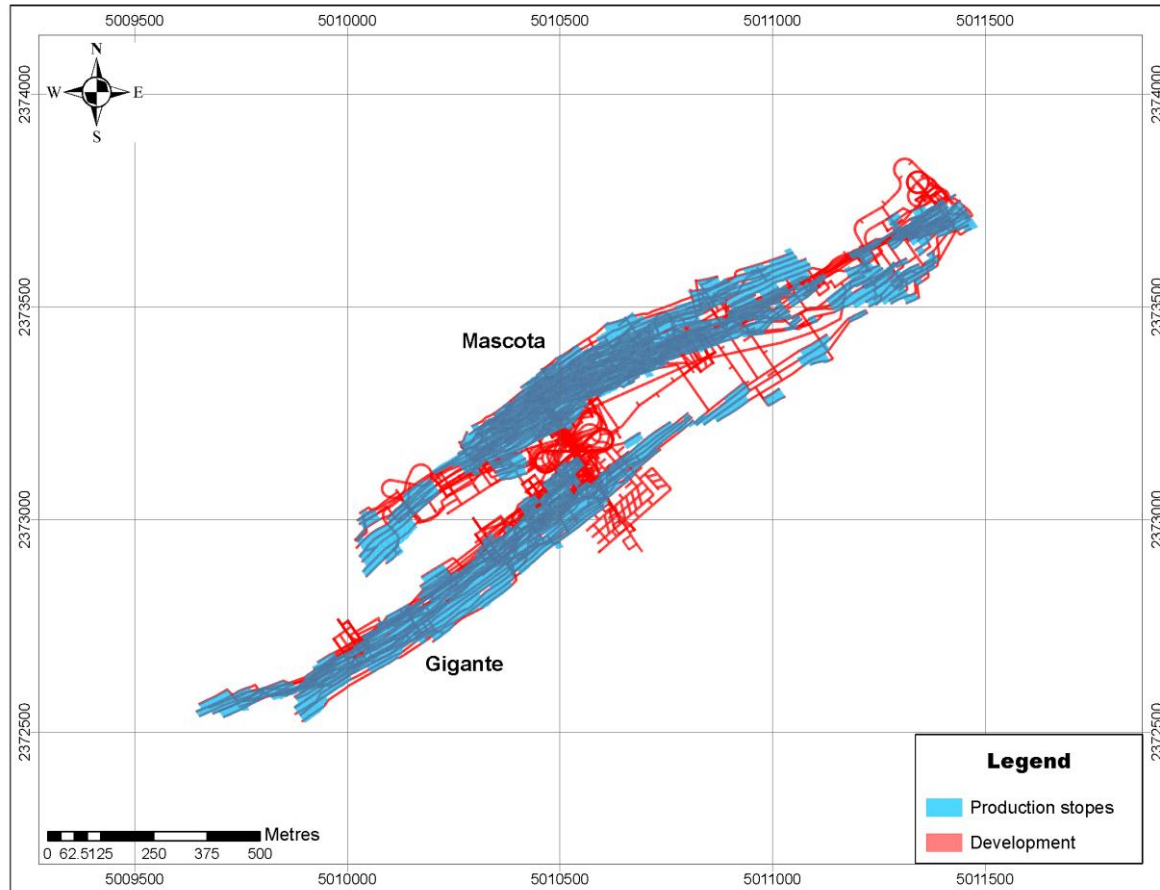
Plan View of Mine Design
