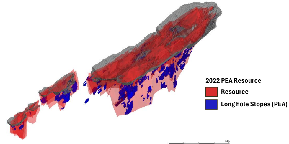
Long Section looking South with Resource and Engineering Designs
