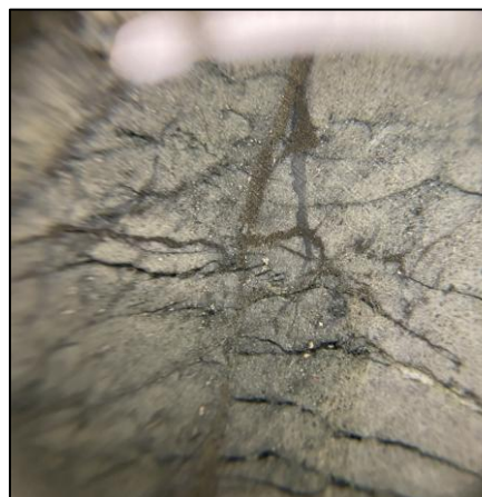
Aiguille: Dark smokey quartz vein with disseminated pyrite mineralization in DUP24-041
