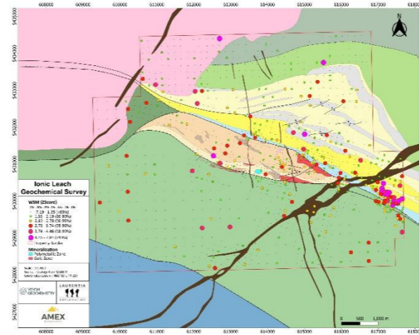
WSM - Soil
