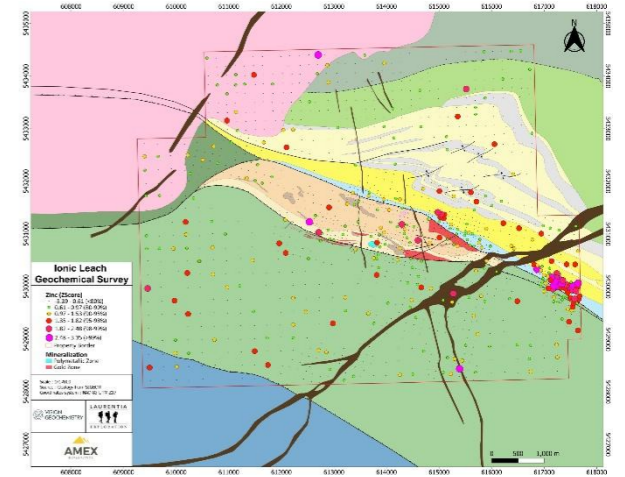
Zn - Soil
