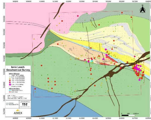
Ag - Soil
