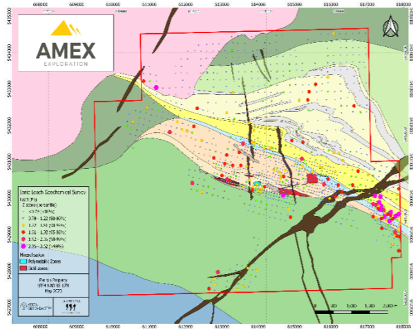
Pb - Soil
