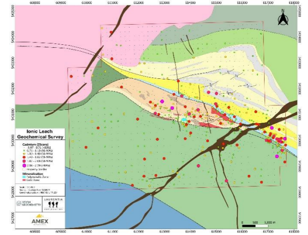
Cd - Soil
